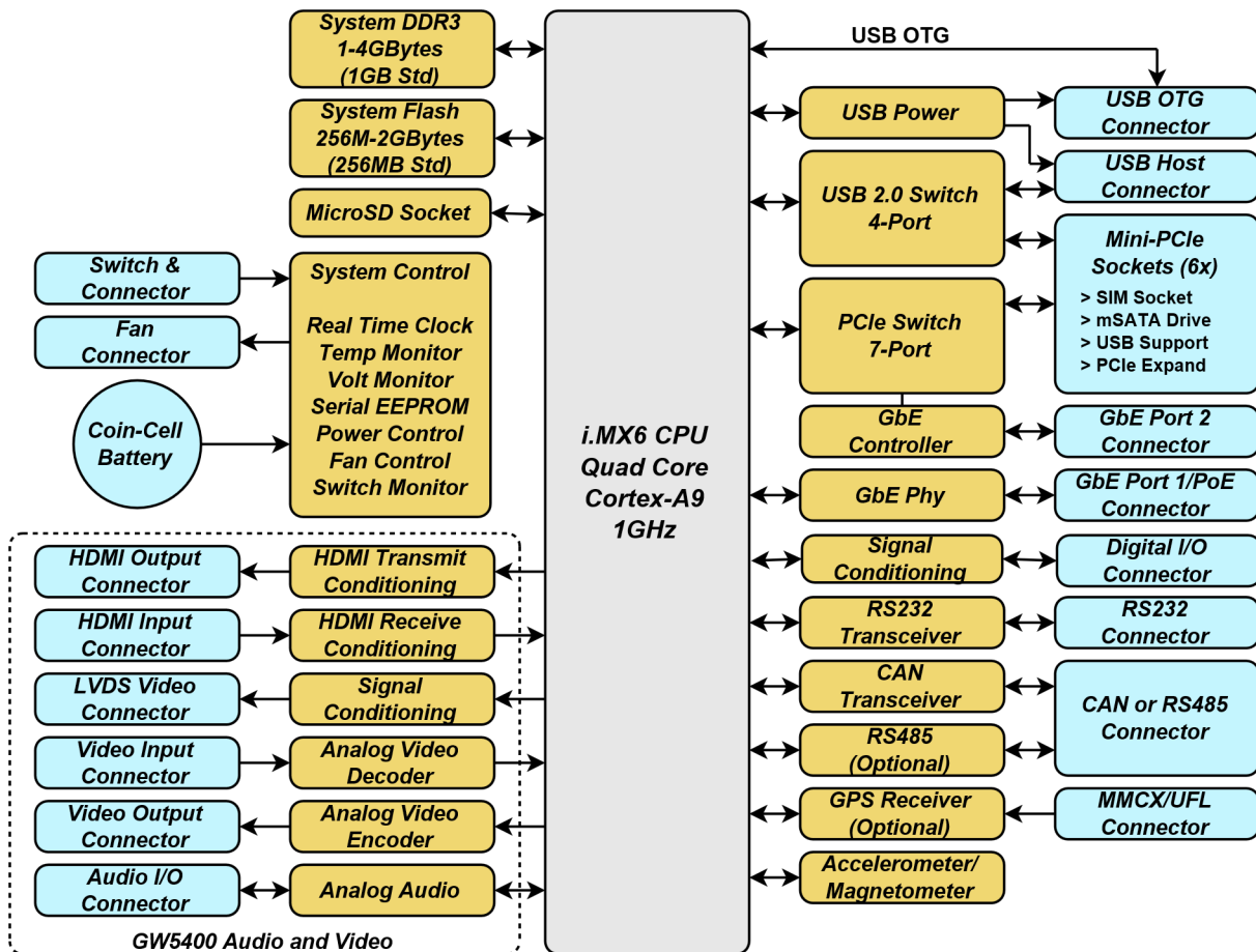
Ventana GW5400 Block Diagram
